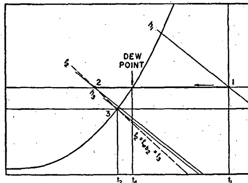
FIG. 8. COOLING OF AIR AT CONSTANT PRESSURE SHOWN ON A.S.H.V.E. PSYCHROMETRIC CHART
