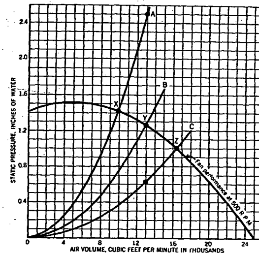
FIG. 5. PARABOLIC SYSTEM CHARACTERISTIC CURVES
