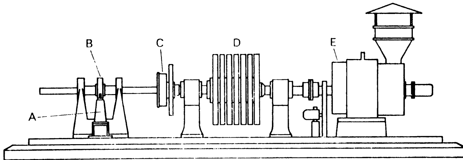
σ 7 / Inertia dynamometer. A: Hydraulic cylinder; B: Torque arm; C: Brake assembly; D: Flywheels; E: Motor.
