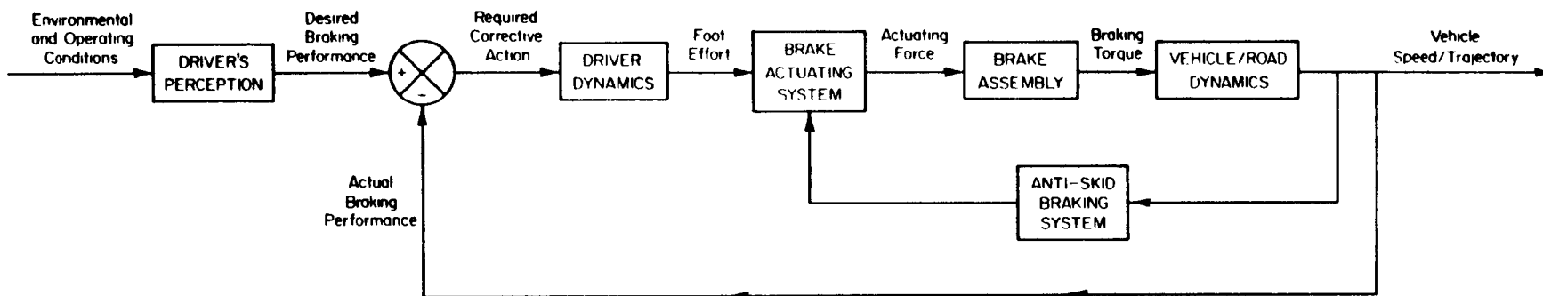
FIGURE 1. SCHEMATIC OF GENERALIZED BRAKING SYSTEM
