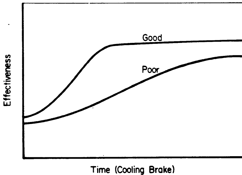
FIGURE 6. FADE RECOVERY CHARACTERISTICS OF GOOD AND POOR BRAKE FRICTION MATERIALS
