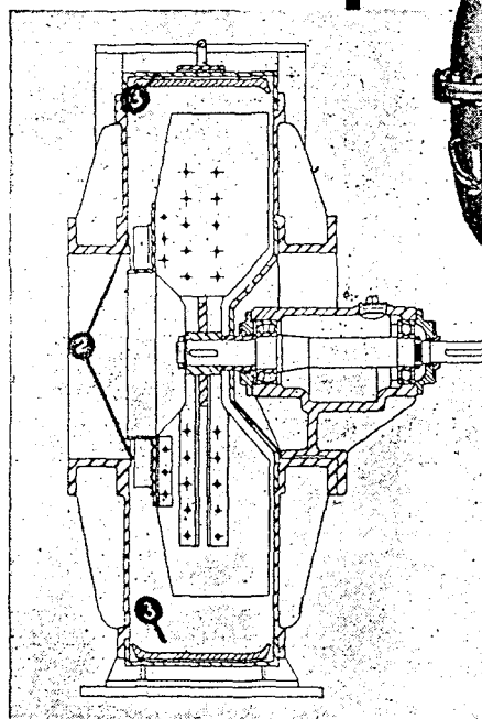
At left — Section through mill exhauster showing new shrouded fan wheel with "whizzer" blades.
