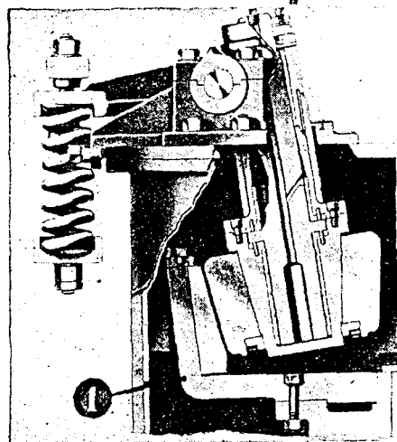
At left — Cutaway view showing section of bowl, grinding ring and roller journal.
