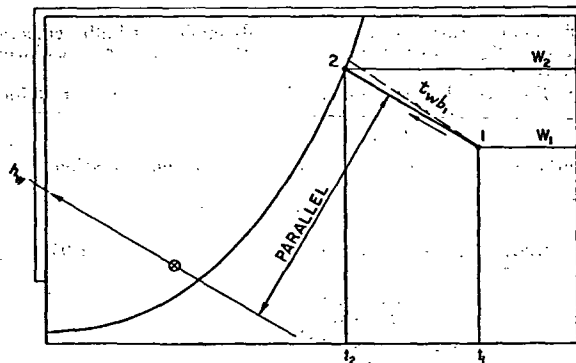
FIG. 13. SOLUTION OF EXAMPLE 6 ON A.S.H.A.E. PSYCHROMETRIC CHART
