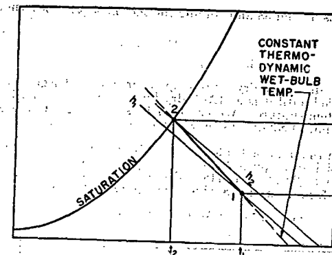
FIG. 14. MOISTURE ADDED AND TEMPERATURE CHANGE
