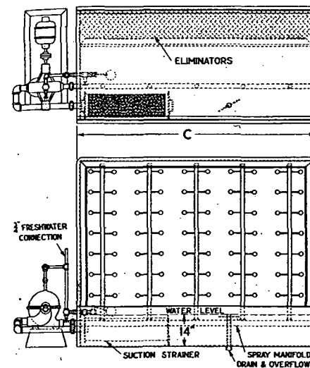
FIG. 1. TYPICAL SINGLE BANK AIR WASHER
