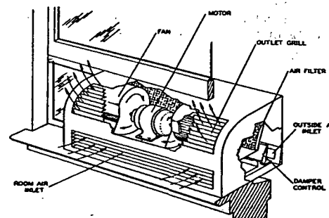
FIG. 12. TYPICAL WINDOW VENTILATOR
