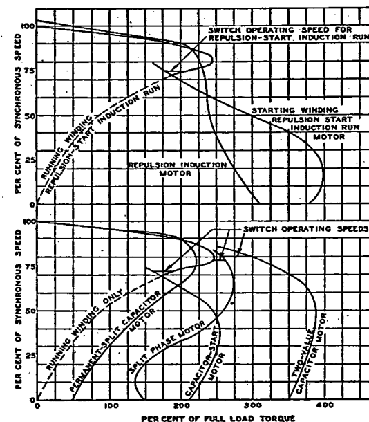
FIG. 3. SPEED-TORQUE CHARACTERISTICS OF SINGLE PHASE MOTORS
