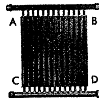
Four connection combinations (A-C, B-D, A-D, B-C) allow tight-spot installation.
