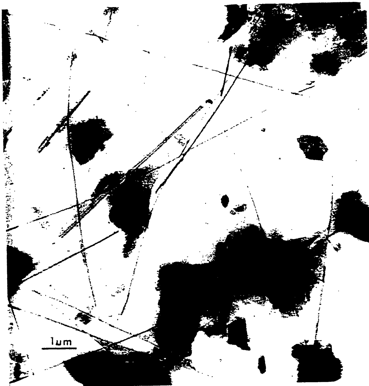
FIGURE 3. Electron photomicrograph of chrysotile-talc (95% talc, 5% chrysotile).
