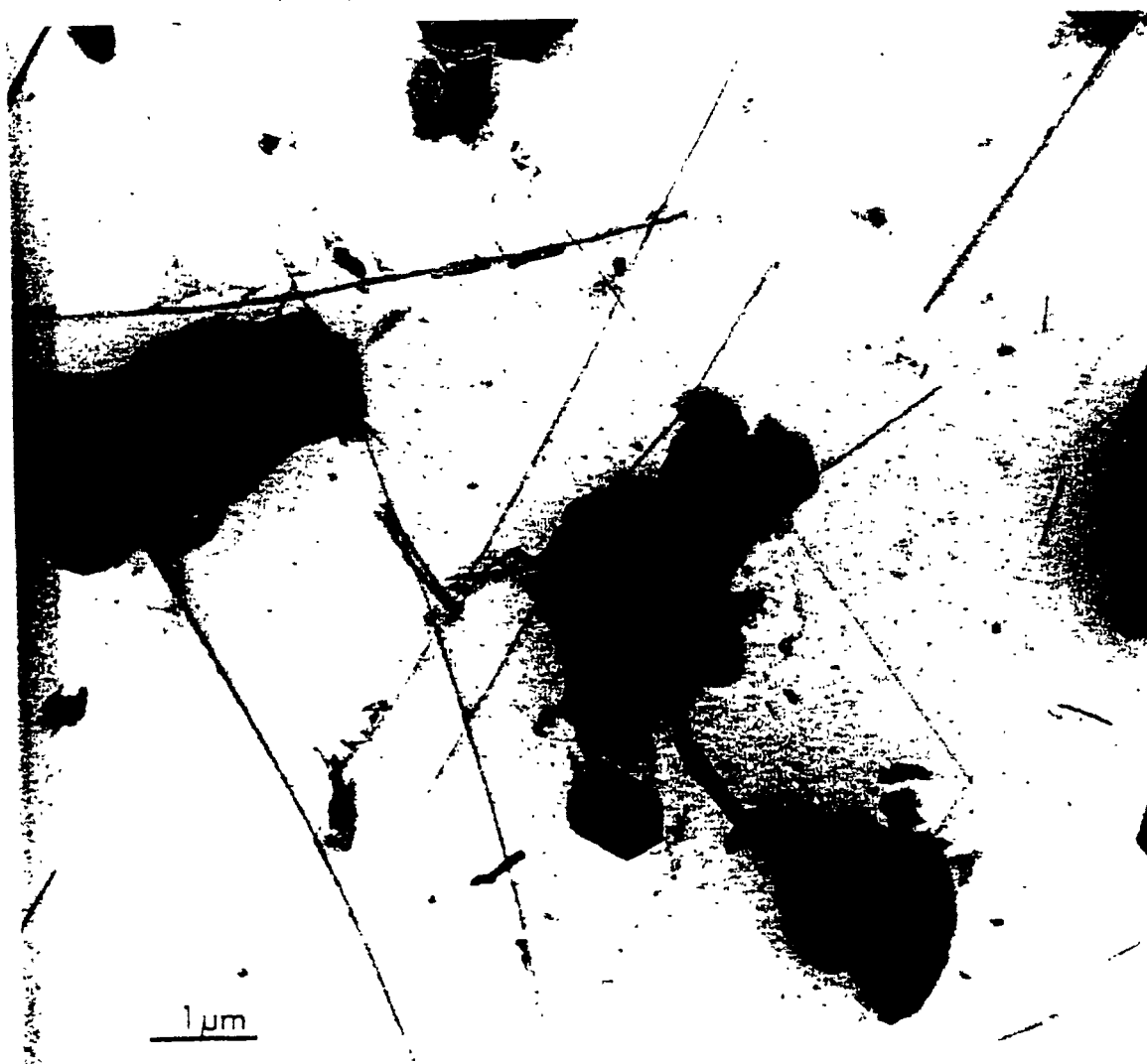
FIGURE 2. Electron photomicrograph of chrysotile-talc (99% talc, 1% chrysotile).
