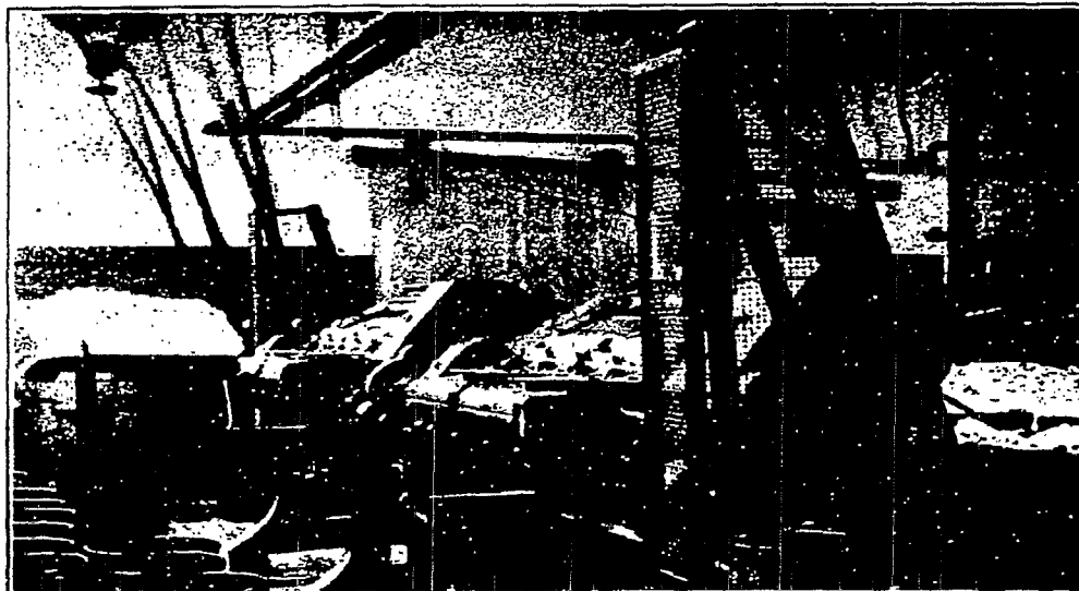
Figure 7. Properly guarded drawing frame, showing guard over combs.
