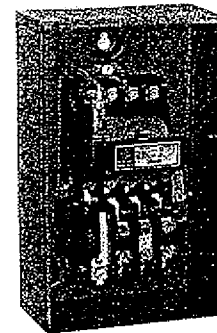
Typical CR206 magnetic motor starter in enclosure with cover removed
