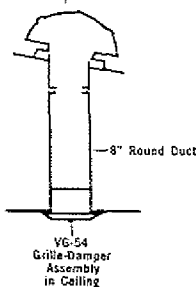
RF-1N Power Ventilator on Roof
