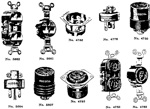
STRAIGHT BLADE 3-WIRE GROUNDING DUPLEX AND SINGLE OUTLETS — SPECIFICATION GRADE 15 Amp., 250 Volts A.C. or D.C.
