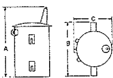
Type HSCA, Self-protected One H-V Bushing
