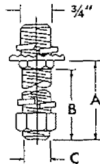
Short Studs — Galvanized Steel
