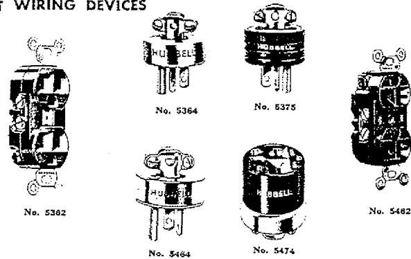
STRAIGHT BLADE 3-WIRE GROUNDING DUPLEX AND SINGLE OUTLETS AND CAPS 20 Amp., 125 Volts A.C. or D.C.
