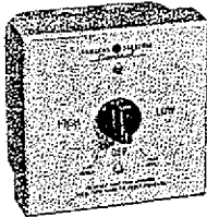
Two-speed NEMA Type 1 enclosed manual starter
