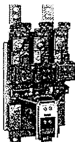
300 ampere electrically held lighting contactor
