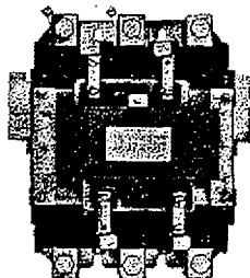
Open 30-, and 300-amp electrically held lighting contactors
