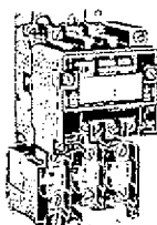
Class 8536 Type SCO-3 Open Type Size 1, 3 pole starter with three thermal units.
