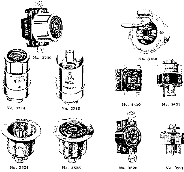
"TWIST-LOCK" 4-WIRE OUTLET, CAP AND CONNECTOR BODY 50 Amp., 250 Volts D.C.; 50 Amp., 600 Volts A.C. With Equipment Ground
