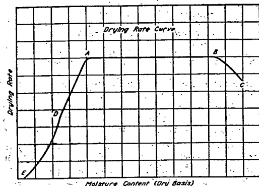
FIG. 3. RATE OF DRYING \frac{dW}{d\theta} VS. MOISTURE CONTENT W
