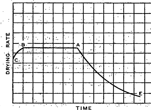
FIG. 4. RATE OF DRYING, \frac{dW}{d\theta} VS. TIME \theta
