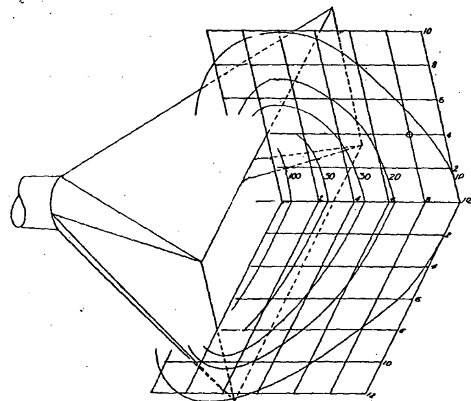
FIG. 1. VELOCITY CONTOURS FOR RECTANGULAR OPENING WITH A SIDE RATIO OF ONE-HALF. CONTOURS ARE EXPRESSED AS PERCENTAGES OF THE VELOCITY AT THE OPENING
