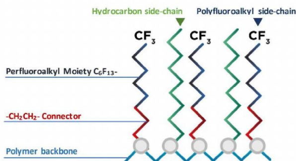
Side-Chain Fluorinated Polymer "comb" structure
