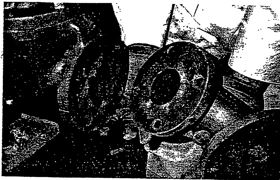
-Photo 4- Removing gasket. Fitting #1B is shown.
