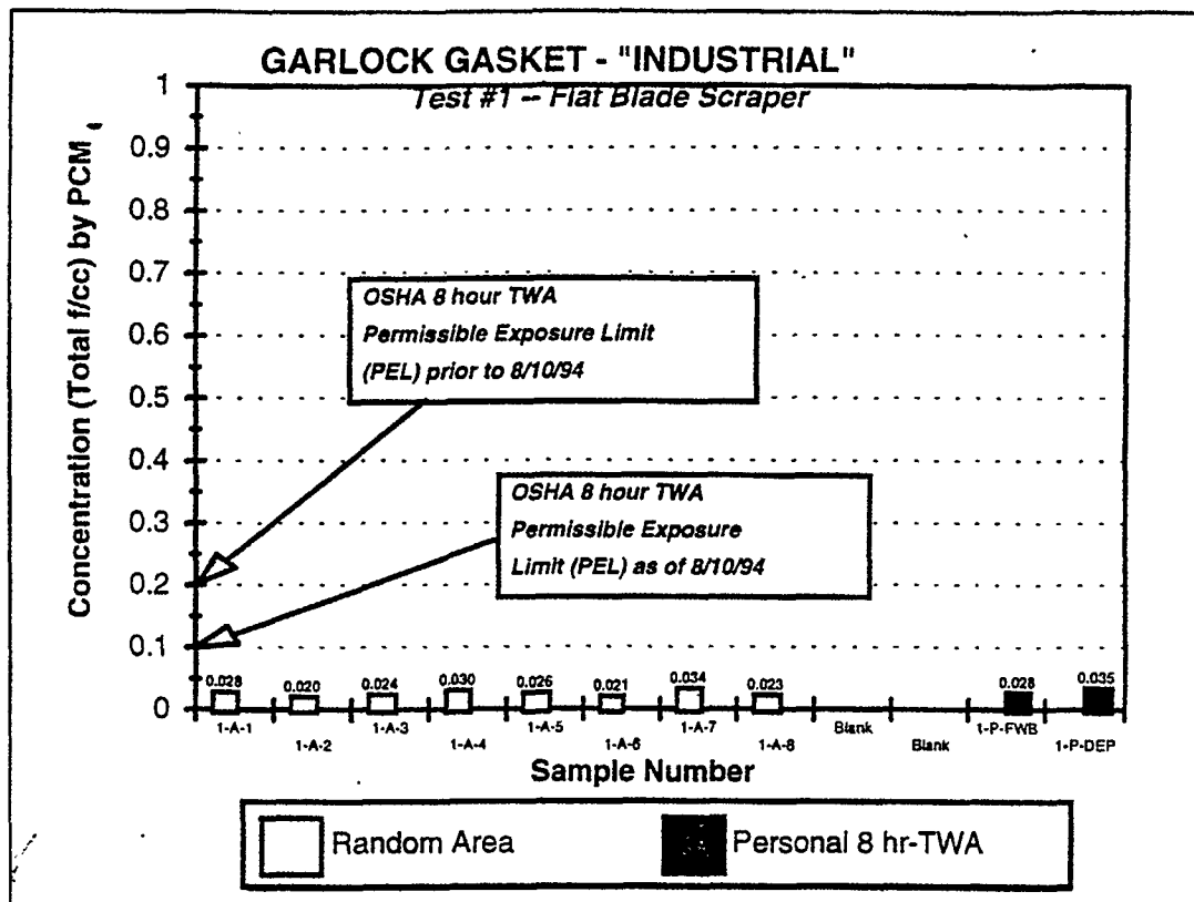
Figure 2 - Graphical presentation of the air sample results.
