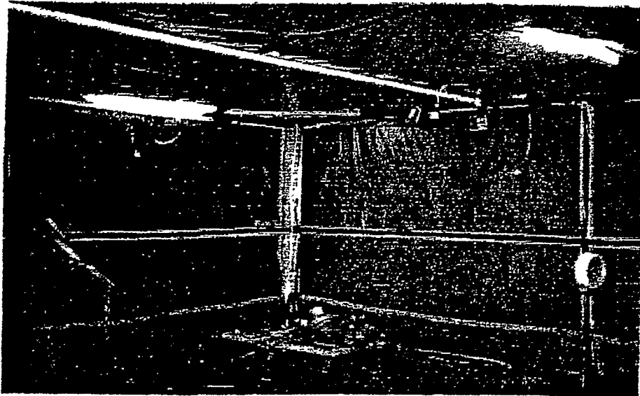
-Photo 1- Test setup for Flat Blade Scraper. Fitting #29B is shown.
