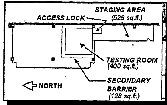
FIGURE 1 - BEC Isolation Test Chamber
