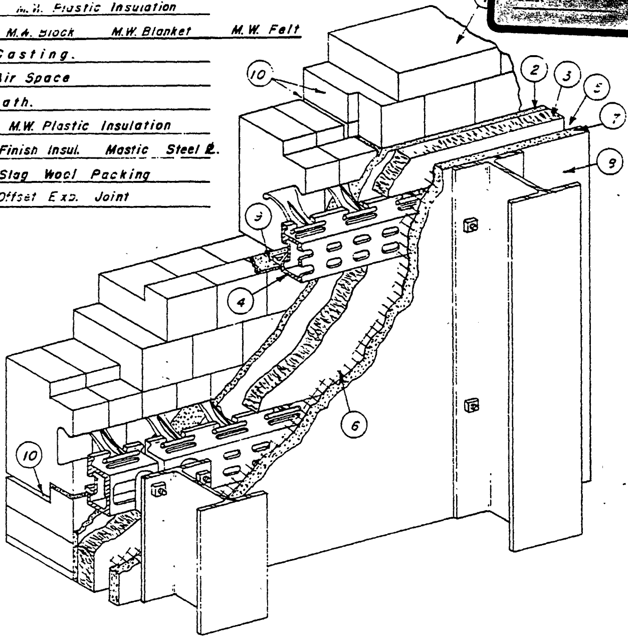
ISOMETRIC OF 7" SEC. SUS. WALL SHOWING INSULATION
