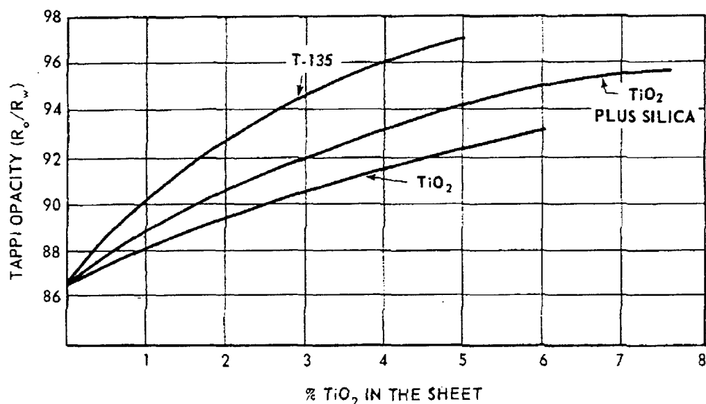
TAPPI OPACITY VS. PER CENT \text{TiO}_2 IN THE SHEET
