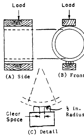
FIG. 2 Assembly for Crushing Strength Test.
