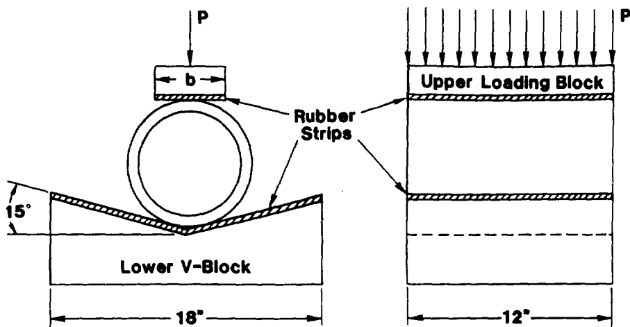
FIG. 3 Assembly for V-Shaped Crushing Strength Test
