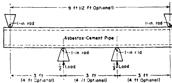
FIG. 1 Assembly for Flexure Strength Test.
