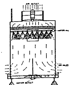
Diagrammatic sketch of Binks Type "K" Tower
