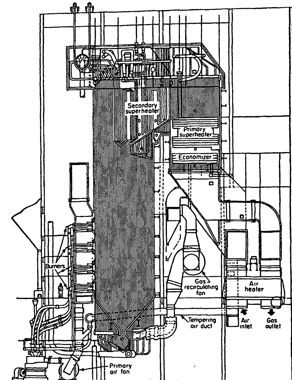
FIG 18-3 – Diagram of large boiler unit shows relative location of auxiliaries This twin-furnace, radiant boiler has circular burners in front wall for pulverized coal Capacity is 2,400,000 lb of steam per hour at 2500 psi and 1050 F/1000 F Hot gases after flowing through the pendent superheater pass downward through the convection pass Hazards to men working on boilers include falls from improper staging, being struck by falling deposits from overhead pipes, asphyxiation or heat prostration, burns from hot equipment, and electric shocks (Note scale of man on boiler operating floor)
