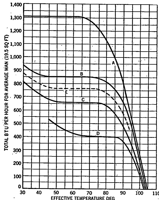
FIG. 5. RELATION BETWEEN TOTAL HEAT LOSS FROM THE HUMAN BODY AND EFFECTIVE TEMPERATURE FOR STILL AIR a 14
