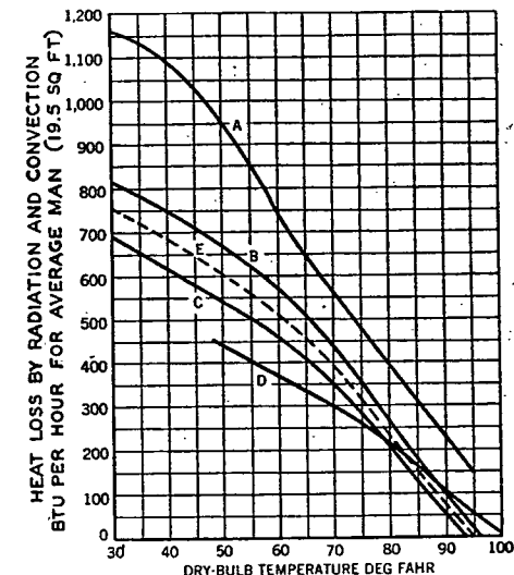
FIG. 6. RELATION BETWEEN RADIATION AND CONVECTION LOSS FROM THE HUMAN BODY AND DRY-BULB TEMPERATURE FOR STILL AIR a 14
