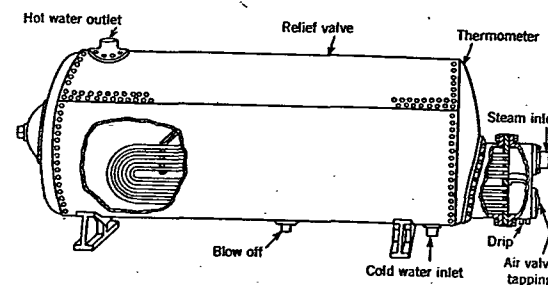
FIG. 8. INDIRECT WATER HEATER
