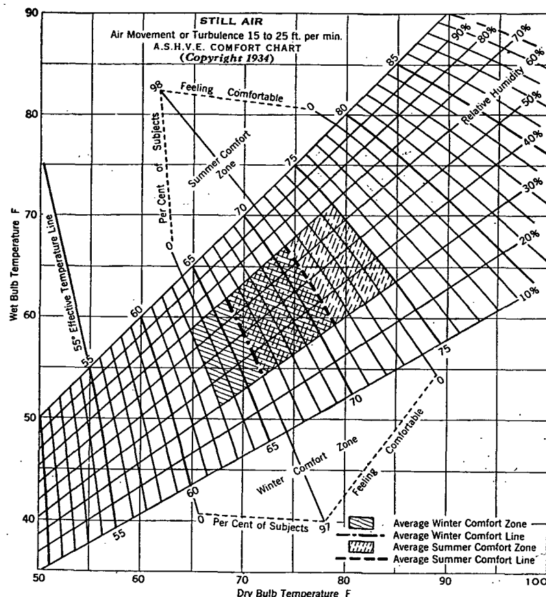
FIG. 6. A.S.H.V.E. COMFORT CHART FOR AIR VELOCITIES OF 15 TO 25 FPM (STILL AIR) 28, 29
