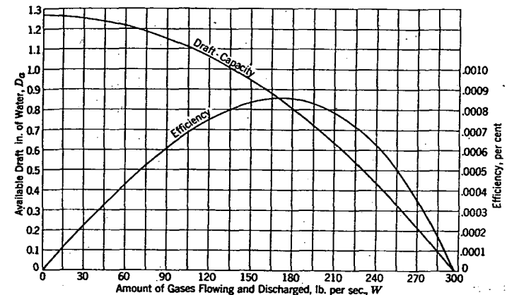
FIG. 4. TYPICAL SET OF OPERATING CHARACTERISTICS OF A NATURAL DRAFT CHIMNEY
