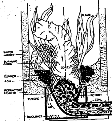
FIG. 9. CROSS-SECTION OF FUEL BED WITH STRONGLY COKING COAL
