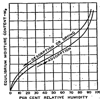
FIG. 5. TYPICAL EQUILIBRIUM MOISTURE CONTENT CURVES 1
