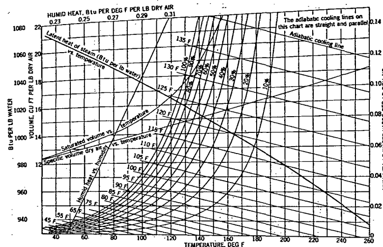
FIG. 6. PSYCHROMETRIC CHART
