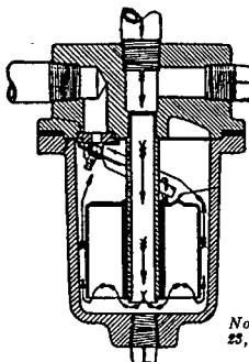
Shows how trap is installed either as an elbow or straight in-line.
