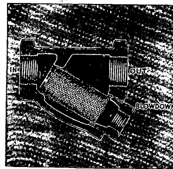
Cutaway view of Anderson strainer
