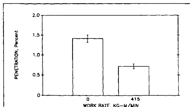
Figure 7. Submicrometer aerosol penetration through a valve compromised with spray paint.
