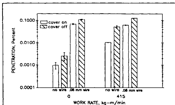
Figure 6. Effect of exhalation valve cover on submicrometer aerosol penetration through exhalation valves. Error bars are one standard deviation ( n = 4 or 5 ).
