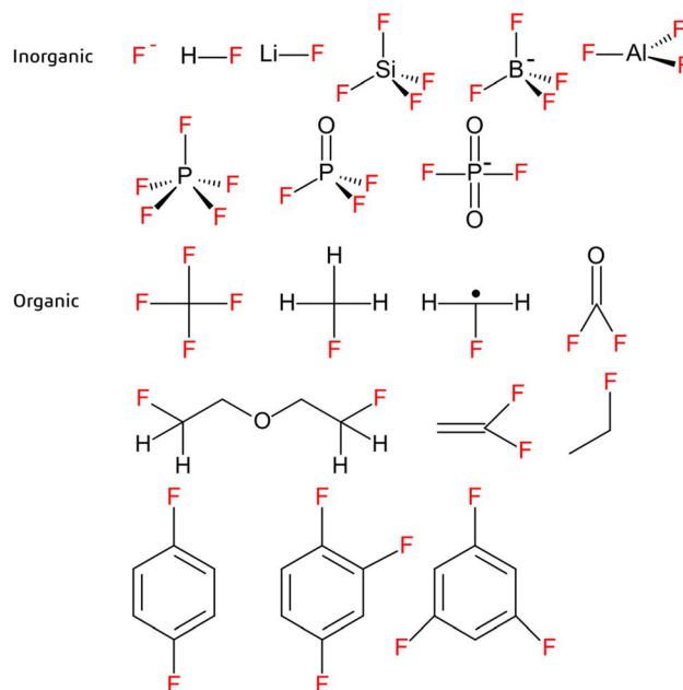
Fig. 4 Examples of inorganic (top) and organic (bottom) fluorinated substances reported in the literature from LIB recycling experiments. 1,3,6,13,16,21,47,53,55,64,72,85,92,94–98.
