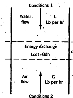
FIG. 4. SECTION OF TYPICAL COUNTER-FLOW TOWER
