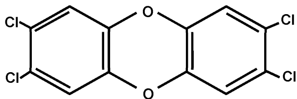
2,3,7,8-Tetrachlorodibenzo-p-dioxin
