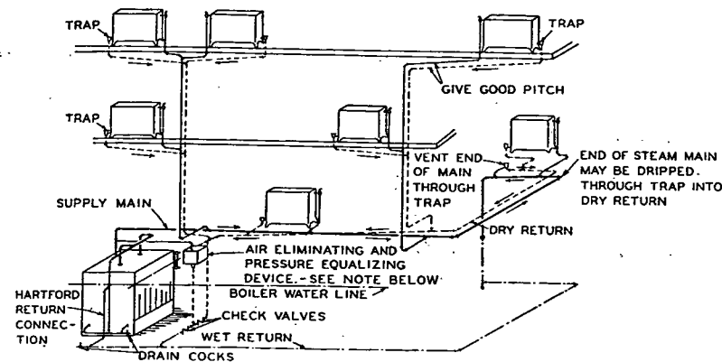
FIG. 11. TYPICAL UP-FEED TWO-PIPE SYSTEM WITH AUTOMATIC RETURN TRAP*
