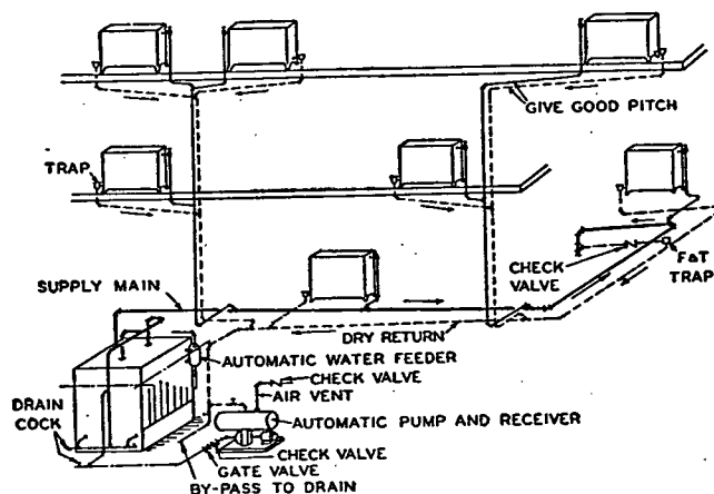
FIG. 10. TYPICAL INSTALLATION USING CONDENSATE PUMP
