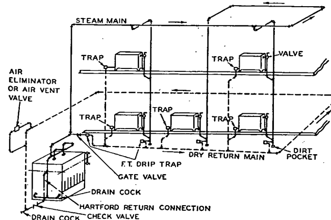
FIG. 12. TYPICAL DOWN-FEED TWO-PIPE SYSTEM
