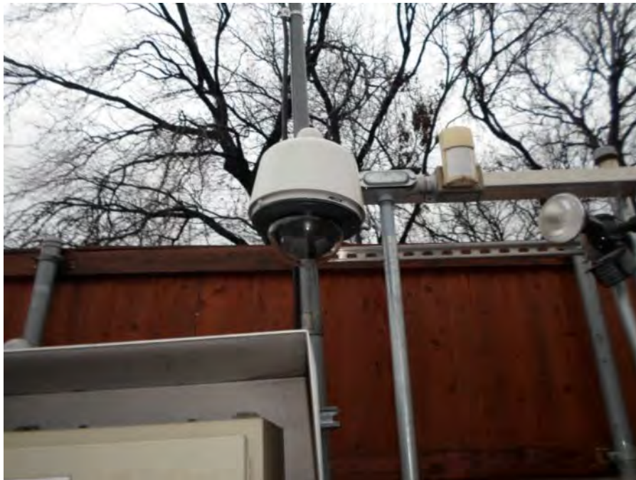
Photograph 12. Meredith Lift Station – View of the station’s security camera, which is connected to the City’s telemetry system and supported by SCADA.
