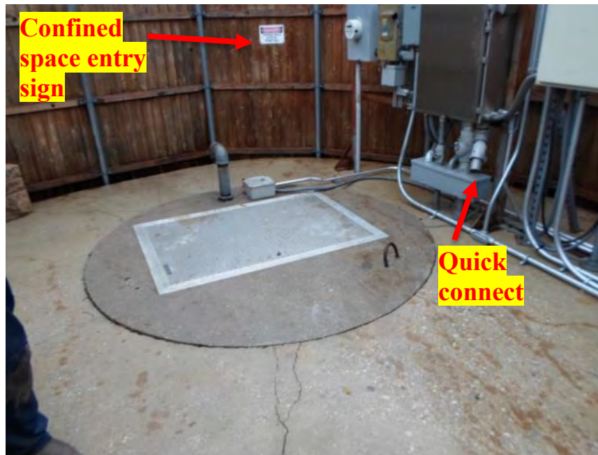
Photograph 40. Clear Creek Lift Station – View of the station's quick connect socket for a portable backup generator and the confined space sign on the fence.
