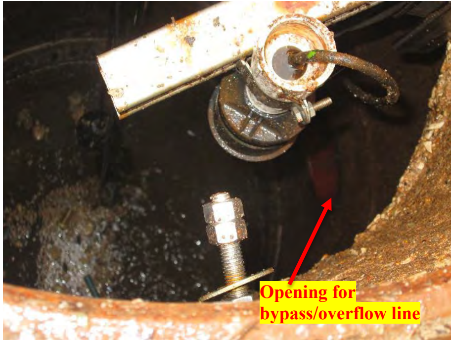
Photograph 15. Meredith Lift Station – View inside the station’s wet well showing the opening where the bypass/overflow line enters from the Collins Lift Station.
