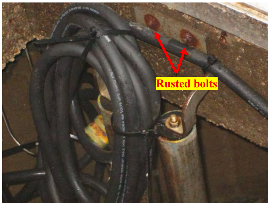
Photograph 42. Clear Creek Lift Station – View of the rusted bolts supporting the pump guide rails at the wet well's access hatch.
