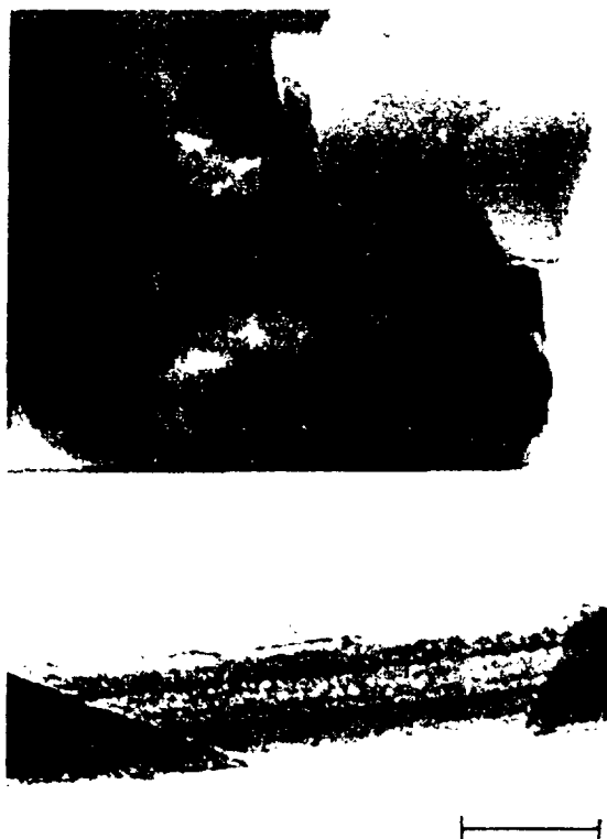
Figure 2. Electron micrographs showing the morphological differences between the amphibole (crocidolite) and the serpentine (chrysotile) types of asbestos. Bar represents 0.05 micrometer.
