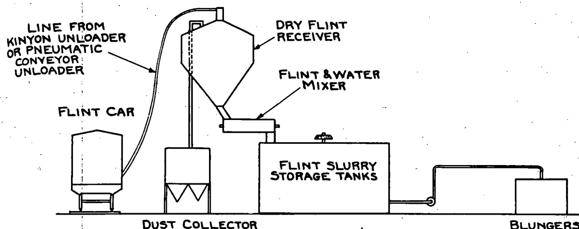
FIG. 1.—Dry flint unloading by pump and storage in form of slurry.
