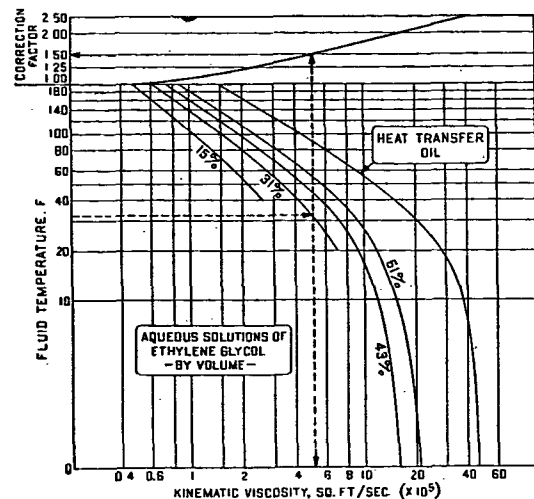
FIG. 21. FRICTION CORRECTION FACTOR FOR VISCOSITY (For N_{Re} > 3000 )
