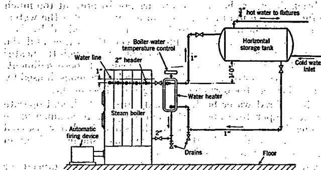
FIG. 9. INDIRECT WATER HEATER MOUNTED ON SIDE OF BOILER
