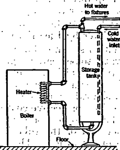
FIG. 10. INDIRECT WATER HEATER PLACED IN BOILER
