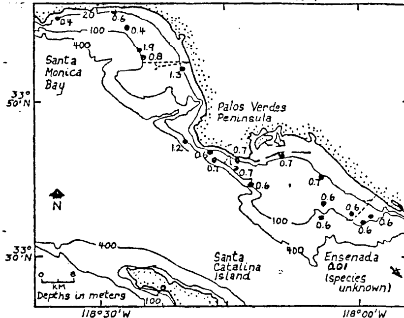
Figure 3. 1254 PCB concentrations (mg/wet kg) in muscle tissue of the crab, Cancer anthonyi , collected off southern California, 1971-72.
