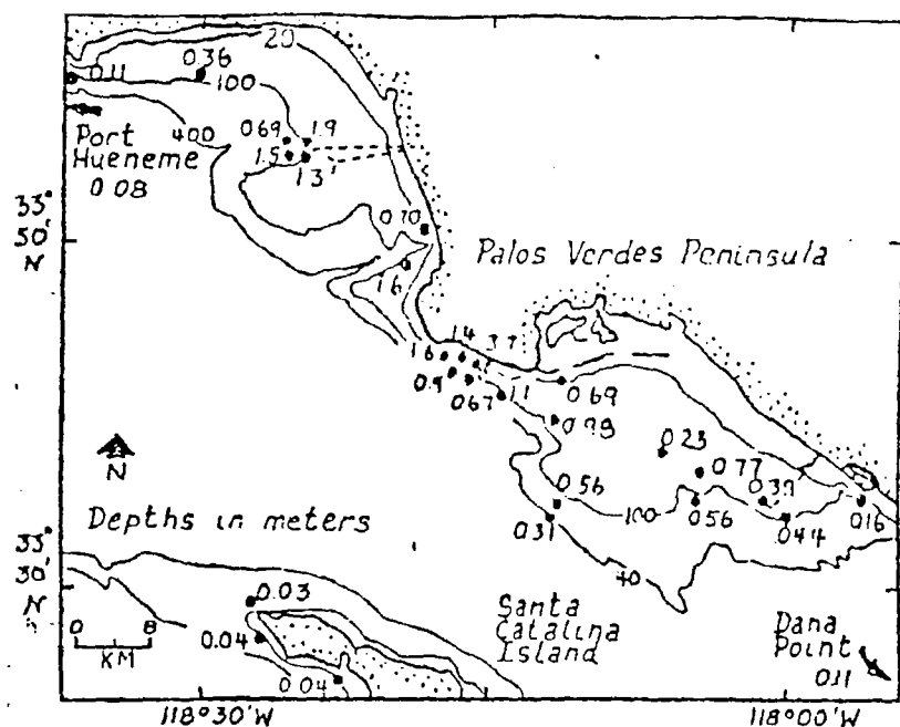
Figure 4. 1254 PCB concentrations (mg/wet kg) in muscle tissue of the Dover sole, Microstomus pacificus , collected off southern California, 1971-72.
