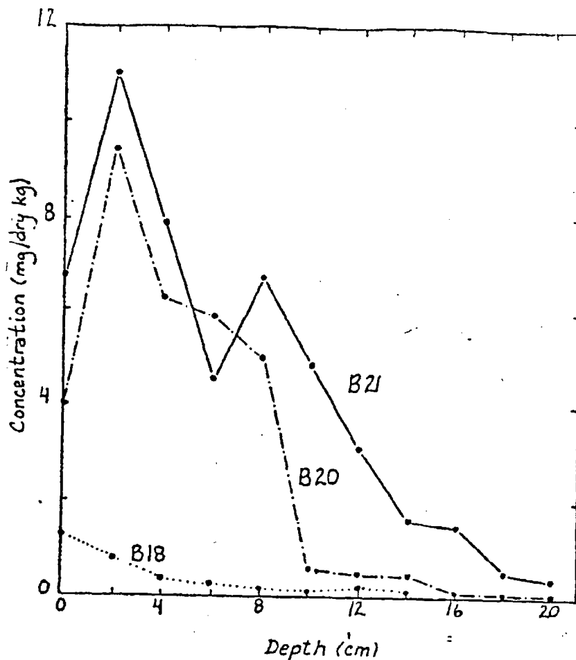
Figure 2. Vertical profiles of 1254 PCB concentrations in sediments collected northwest of the JWPCP outfalls, box cores, July 1971.
