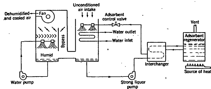
FIG. 9. OPEN LIQUID ADSORPTION SYSTEM
