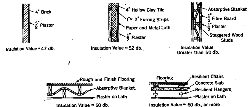
FIG. 2. THREE WALL SECTIONS AND TWO FLOOR AND CEILING SECTIONS WHICH ARE SUITABLE FOR THE INSULATION OF EQUIPMENT ROOMS*
