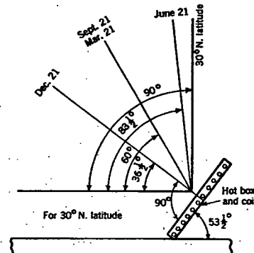
FIG. 13. SOLAR HEATING COIL INCLINATION
