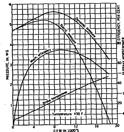
FIG. 2. GENERAL OPERATING CHARACTERISTICS OF TYPICAL INDUCED DRAFT FAN
