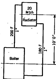
FIG. 7. GRAVITY SYSTEM
