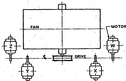
Location of motor is determined by facing the drive side of fan or blower and designating the motor position by letters W, X, Y or Z as the case may be.
