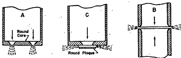
FIG. 1. CROSS-SECTIONS OF ROUND DUCTS WITH THREE BASIC TYPES OF ANNULAR OUTLETS.
