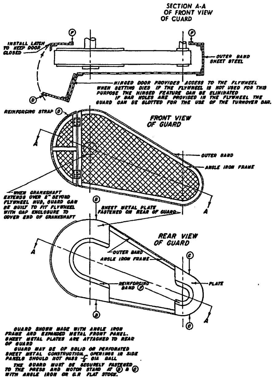
Fig. 22-8. A well-designed flywheel guard for individually driven machines. This type of guard gives excellent protection and easy access to wheel for adjustments or repair.
