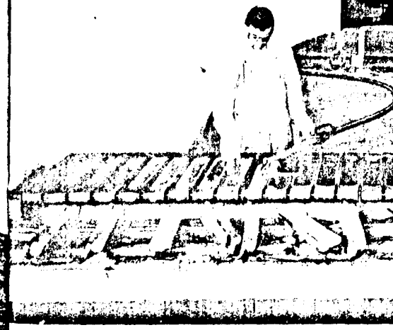
Right: Tapping-off molten metal from secondary metal blast furnace. Below: After removal of other metals such as copper and tin, the lead is run into molds for casting into pigs.
