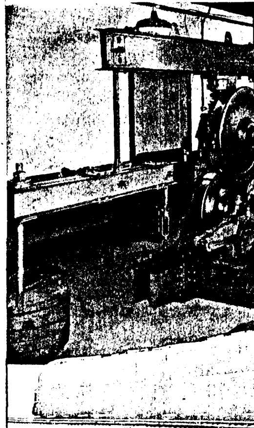
Journal bearing testing machine installed in the Division for making tests on journal boxes and wheel speeds up to 90 miles per hour.
