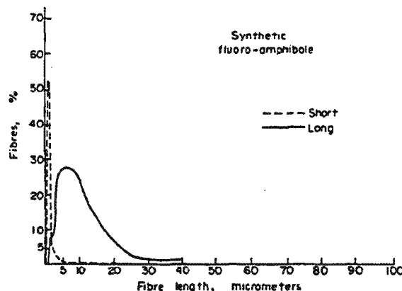
FIG. 5. Schematic representation of fibre lengths of short and long samples of a synthetic fluoramphibole.
