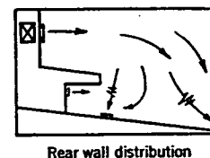
FIG. 8. AIR DISTRIBUTION METHODS FOR THEATERS, CHURCHES, AND AUDITORIUMS
